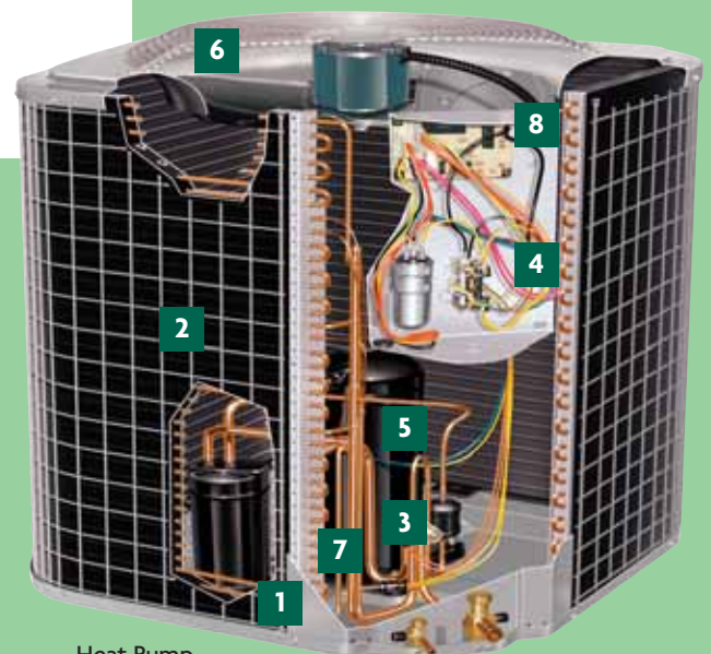
Heat Pump
